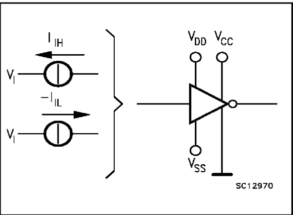
FIGURE 2: Driver Test Circuit for I IH and I IL
