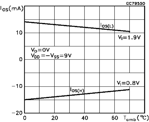
Driver Short Circuit Output Current vs Free-Air Temperature
