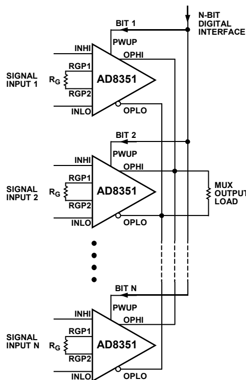
Figure 42. Using Several AD8351 s to Form an N-Channel Analog MUX
