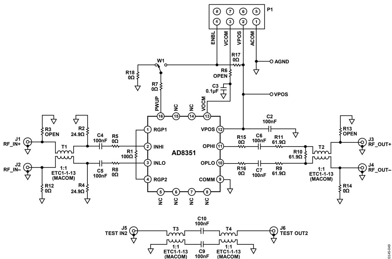
Figure 50. Evaluation Board Schematic
