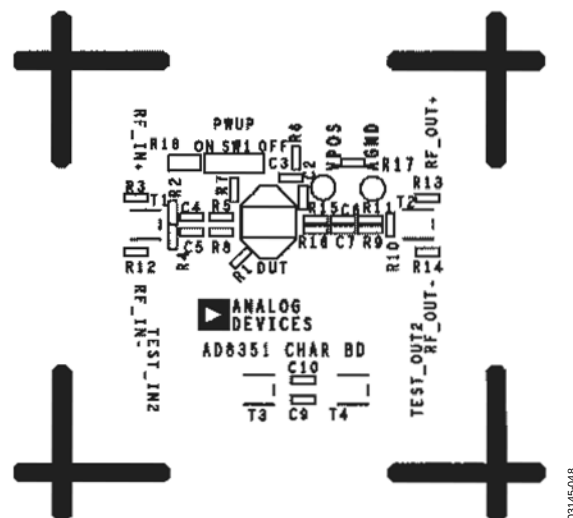
Figure 49. Component Side Silkscreen
