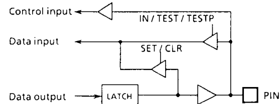
Figure 3-5. Port R8
