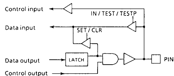
Figure 3-6. Port R9
