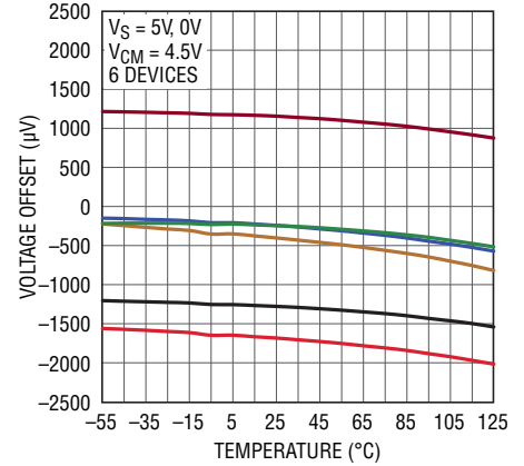
V_{OS} vs Temperature (MS10, NPN Stage)
