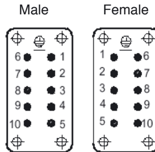
view from cable side
