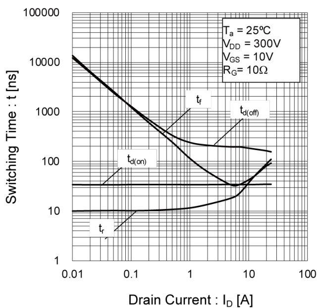
Fig.18 Switching Characteristics
