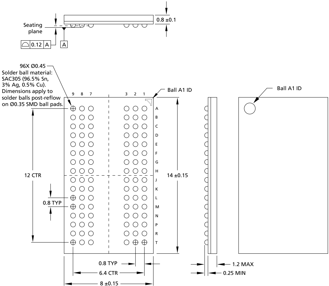
Figure 4: 96-Ball FBGA – x16 (JT)
