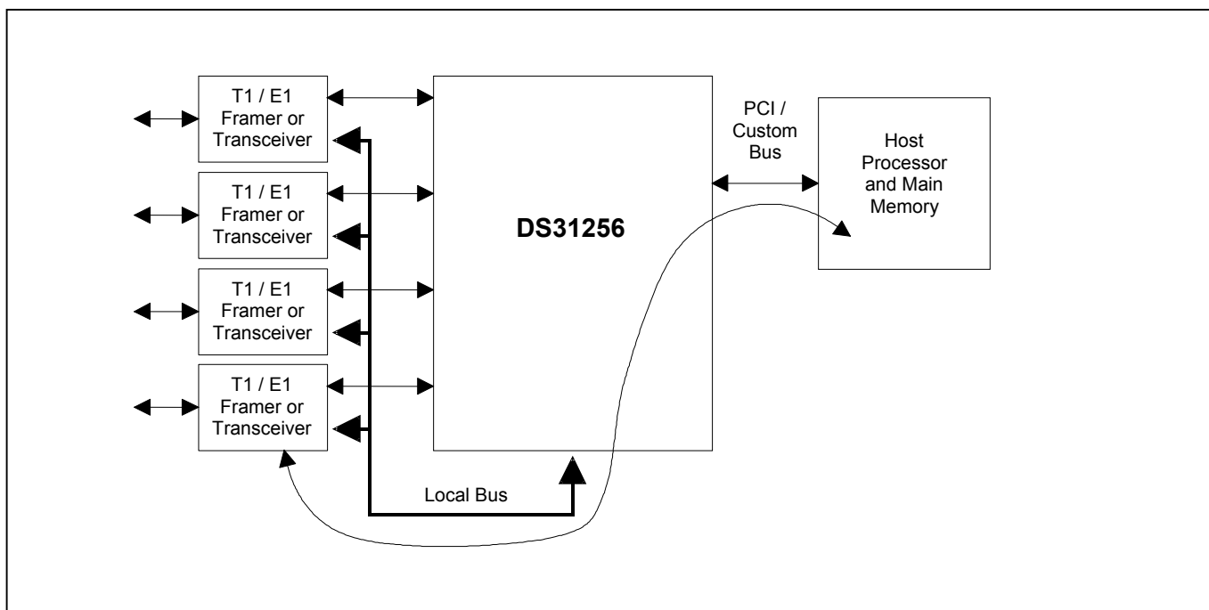
Figure 11-1. Bridge Mode
