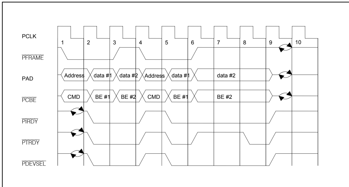
Figure 10-9. PCI Fast Back-To-Back
