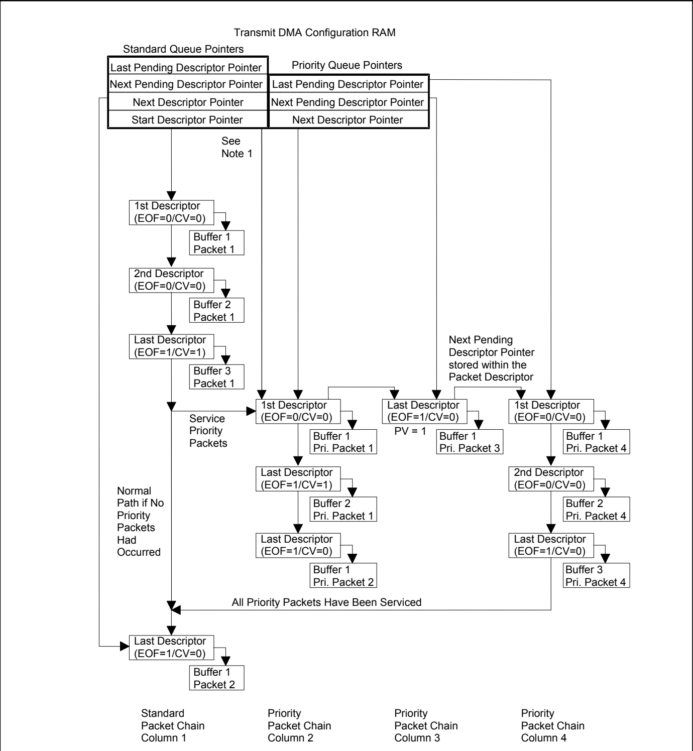
Figure 9-13. Transmit DMA Priority Packet Handling
