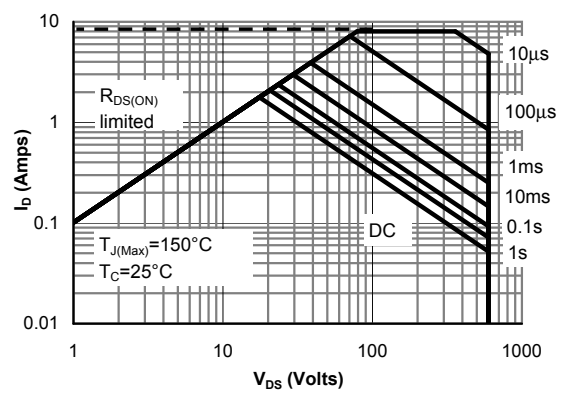
Figure 10: Maximum Forward Biased Safe Operating Area for AOTF2N60 (Note F)
