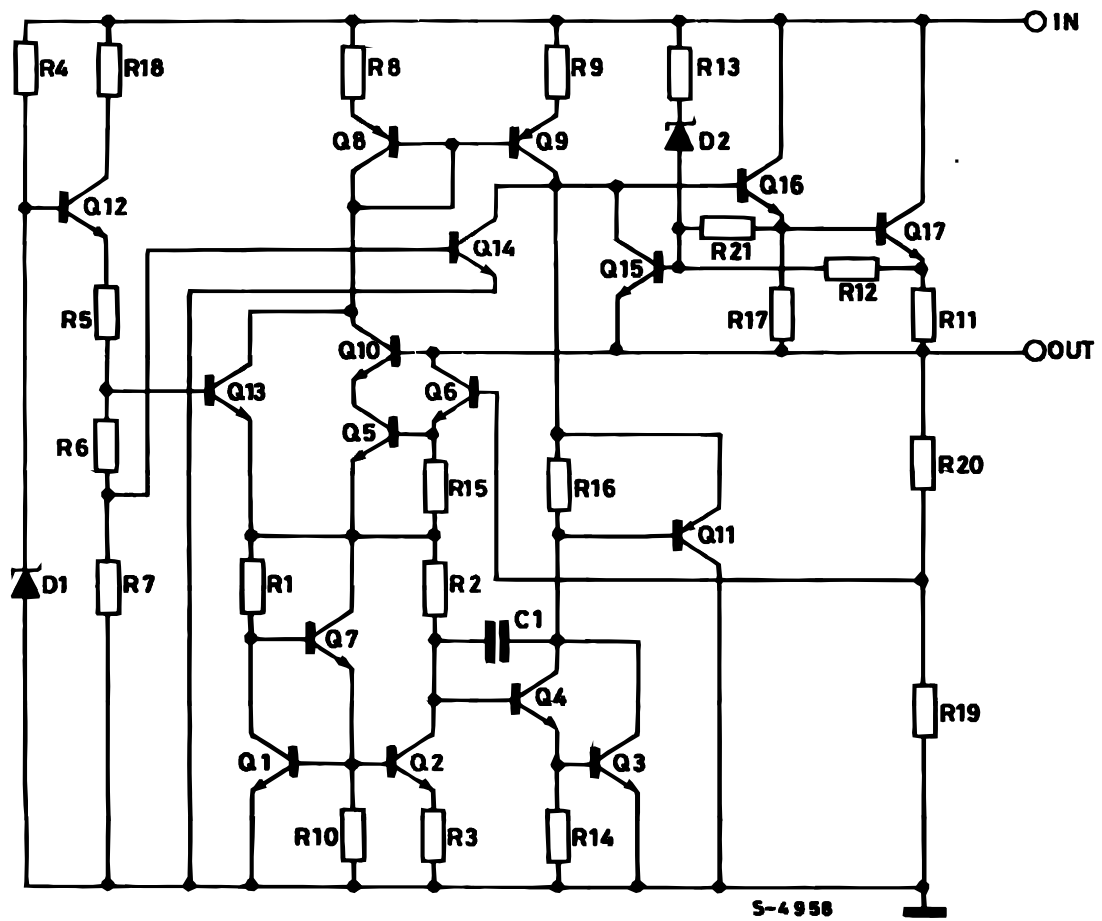
Figure 3. Schematic diagram
