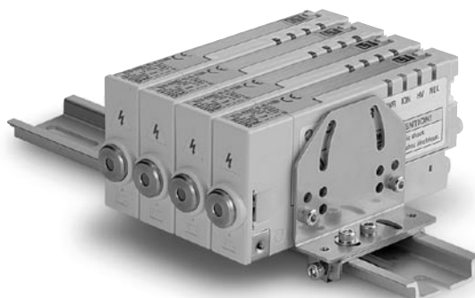
Manifold*
