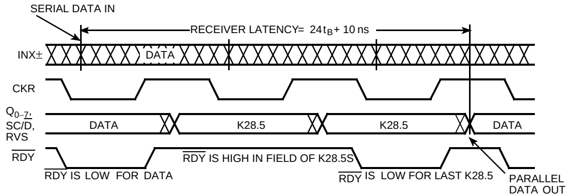
Figure 5. CY7B933 Framing Operation in Encoded Mode
