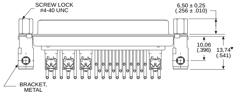
Engaging Face
