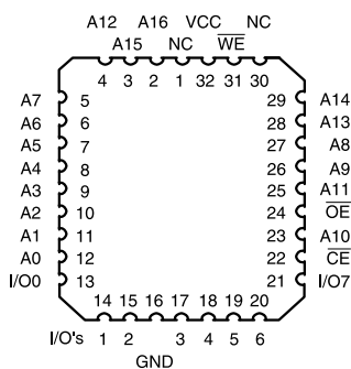
PLCC Top View
