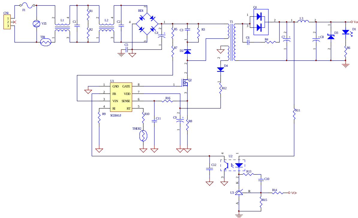
Figure 15. Reference Circuit
