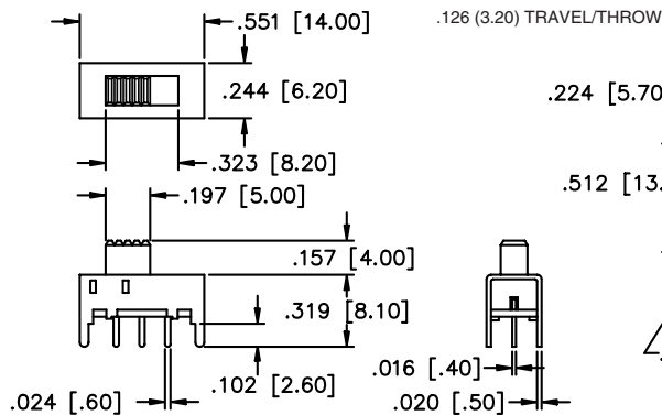
MECHANICAL OUTLINE
