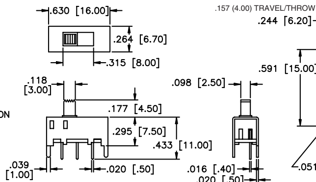
MECHANICAL OUTLINE
