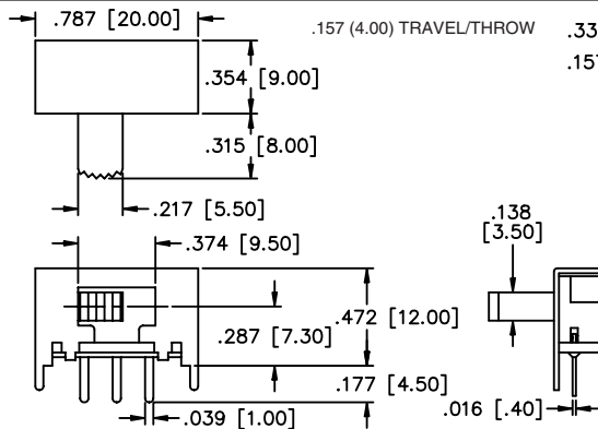
MECHANICAL OUTLINE
