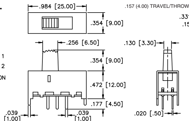
MECHANICAL OUTLINE
