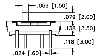
MECHANICAL OUTLINE
