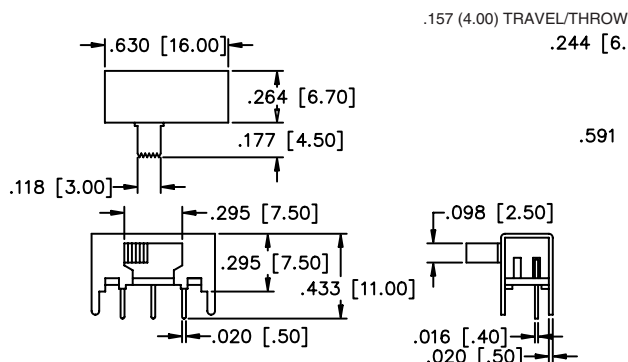
MECHANICAL OUTLINE
