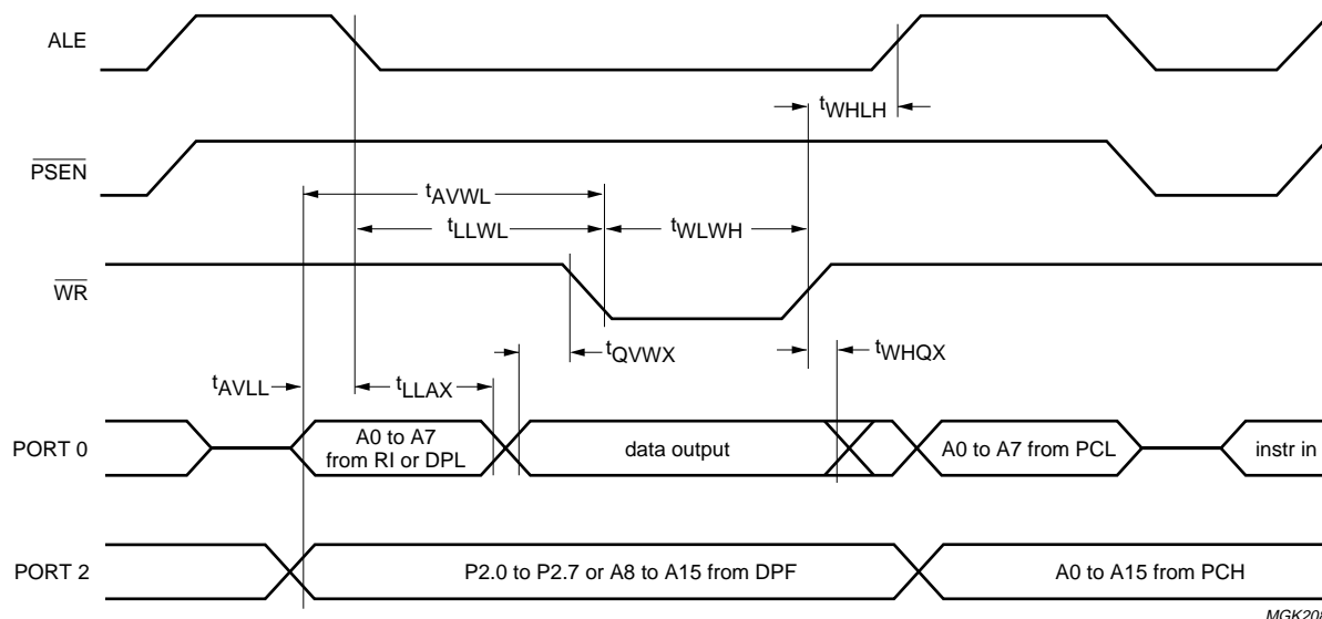
Fig.35 External data memory write cycle.
