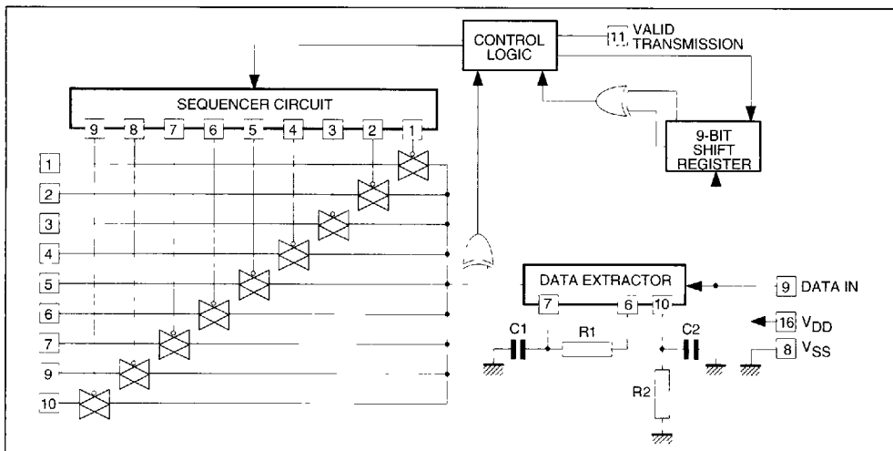
Figure 3 : Decoder M145028
