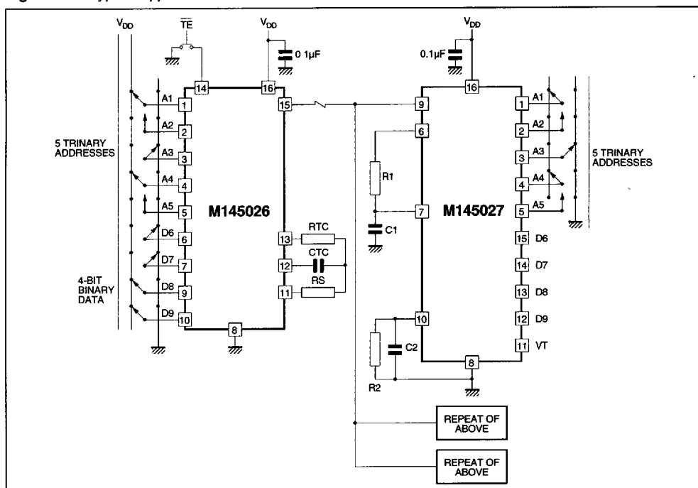
Figure 10 : Typical Application
