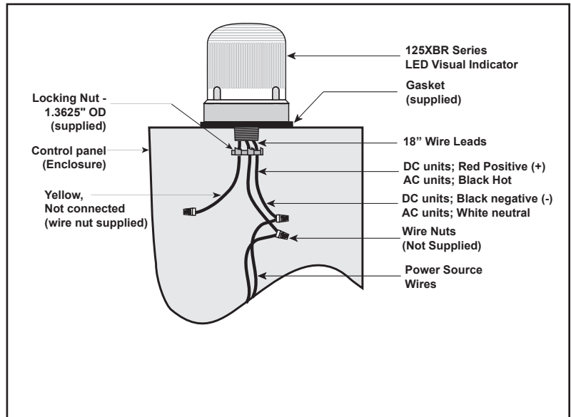
Figure 2. Panel Mounting
