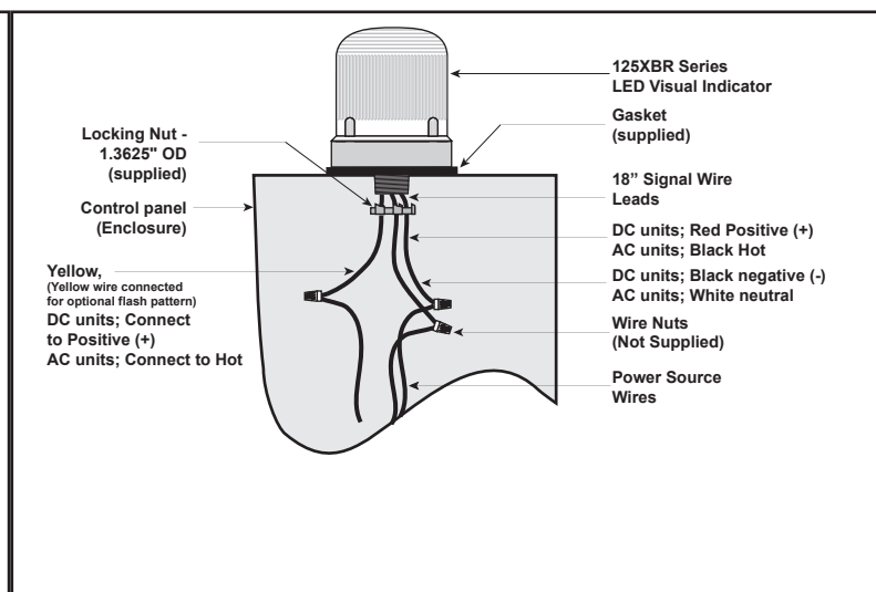
Figure 4. Panel Mounting
