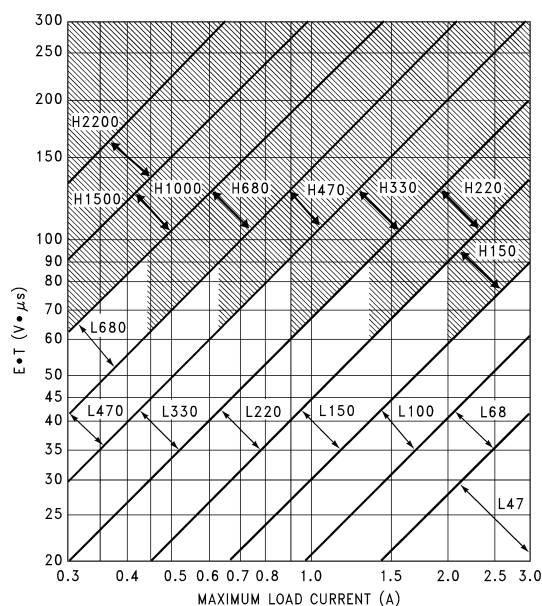
FIGURE 7. LM2576(HV)-ADJ
