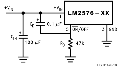
FIGURE 14. Delayed Startup
