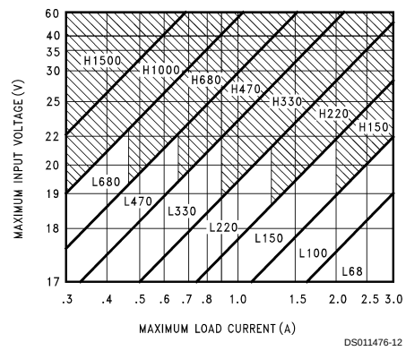
FIGURE 6. LM2576(HV)-15
