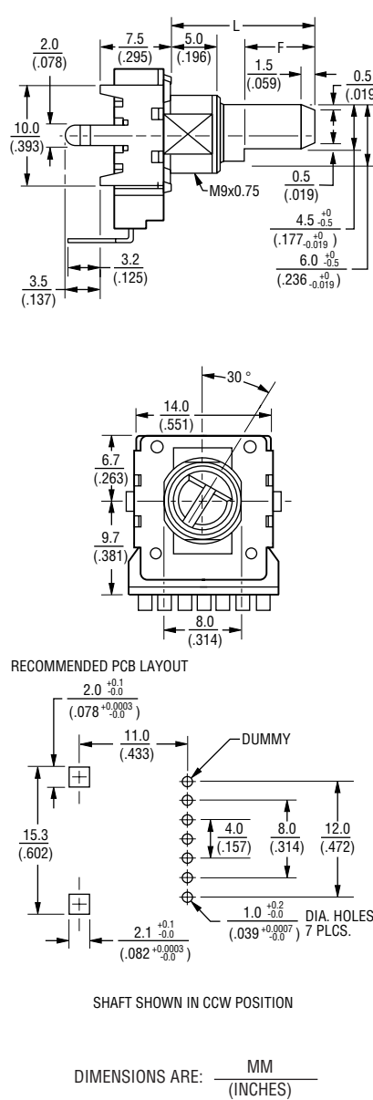
PTV142B-4 With Bushing
