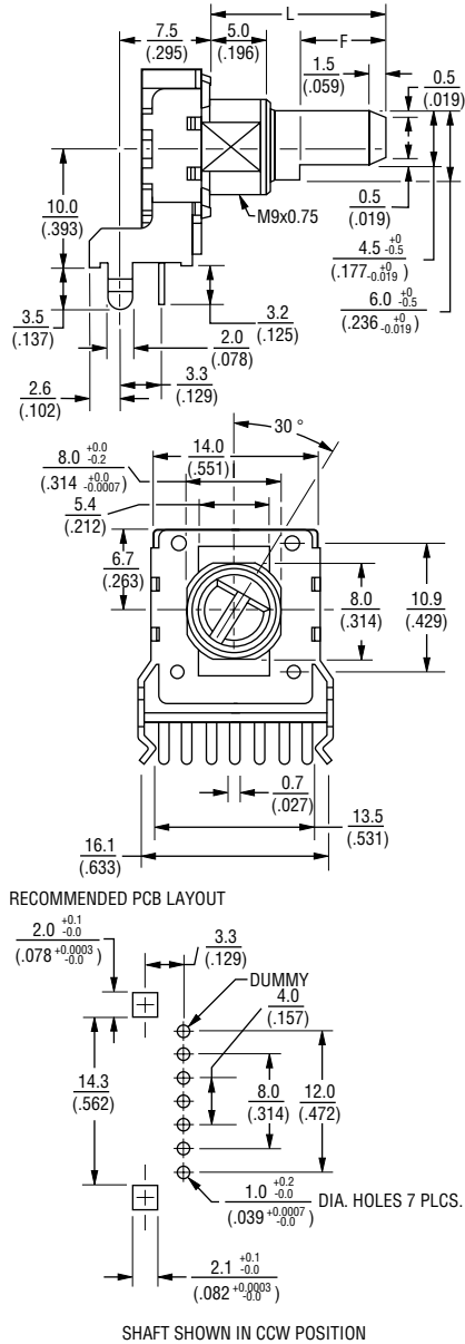
PTV142B-2 With Bushing
