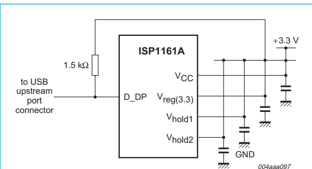
Fig 44. Using a 3.3 V supply.
