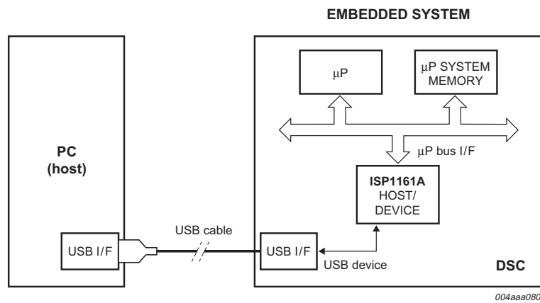
Fig 1. ISP1161A operating as a USB device.
