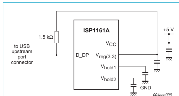
Fig 43. Using a 5 V supply.
