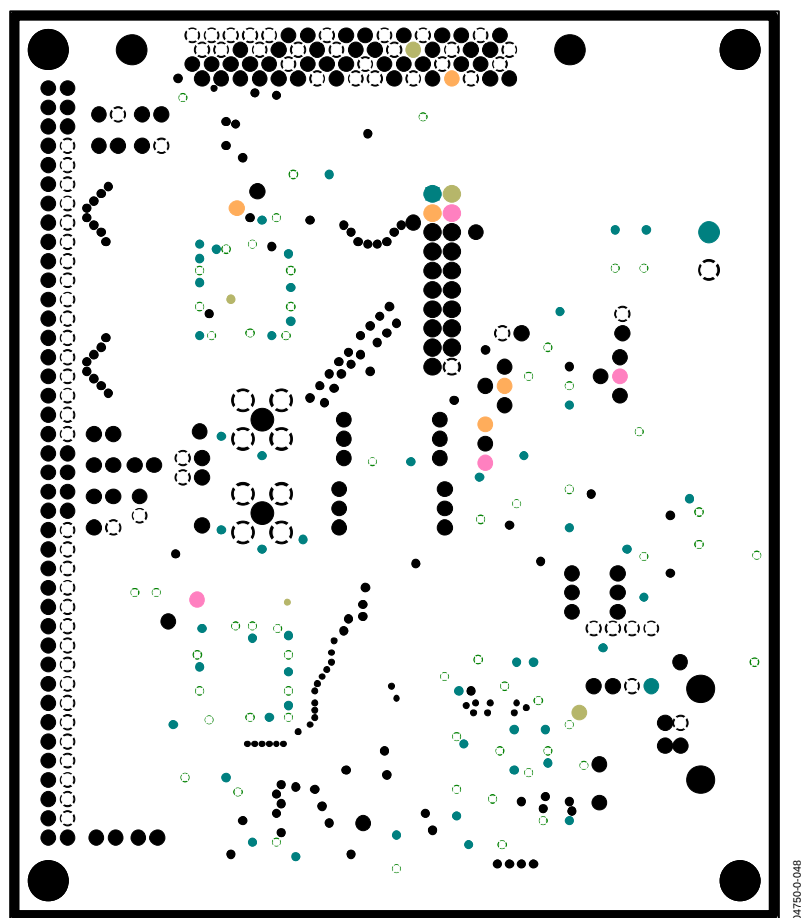
Figure 37. Layer 2—Ground Plane
