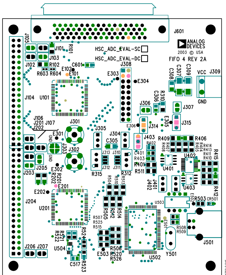
Figure 34. Assembly—Primary Side
