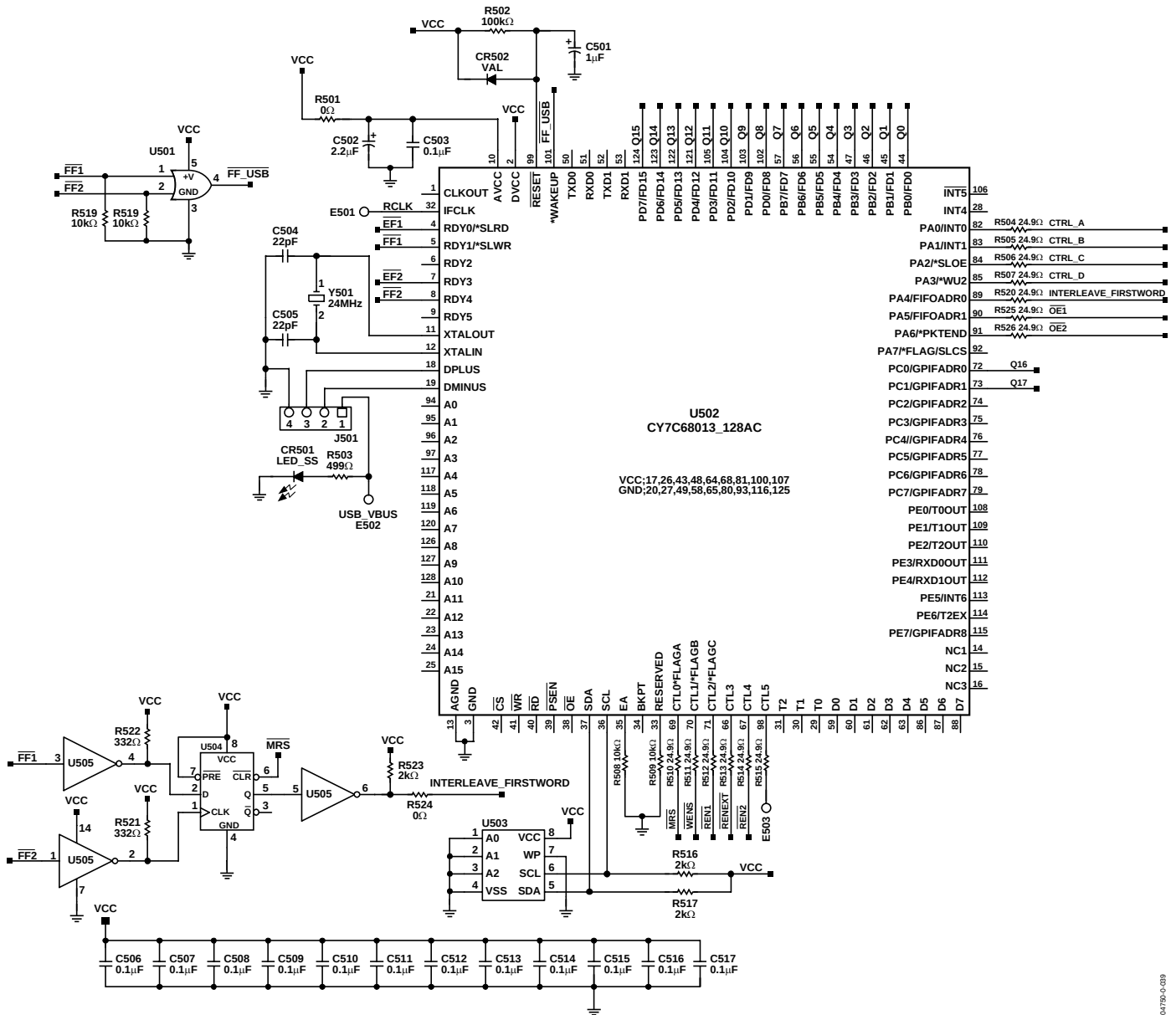
Figure 28. PCB Schematic
