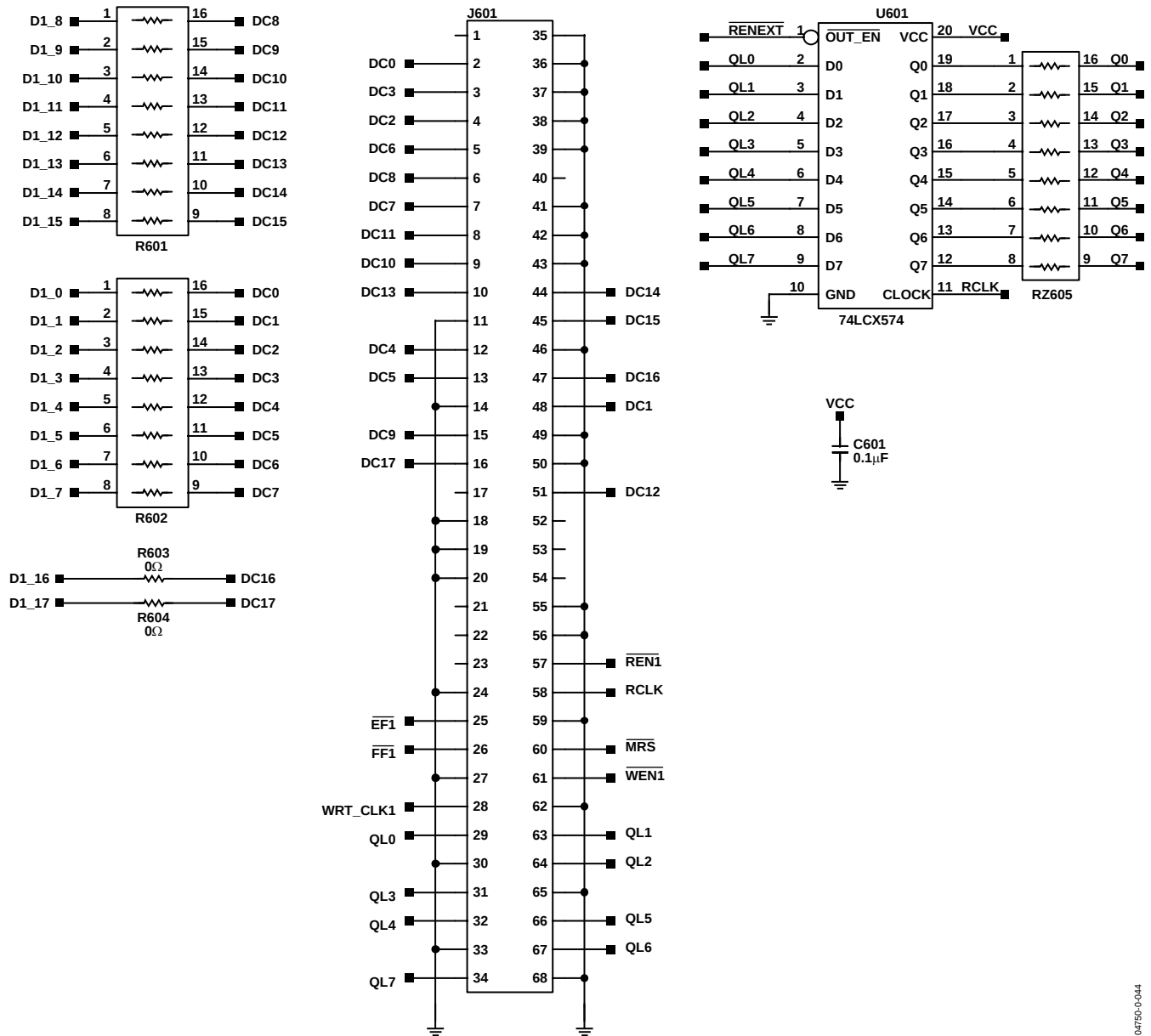
Figure 33. PCB Schematic (Continued)
