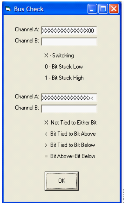
Figure 18. Bus Check for a 12-Bit ADC
