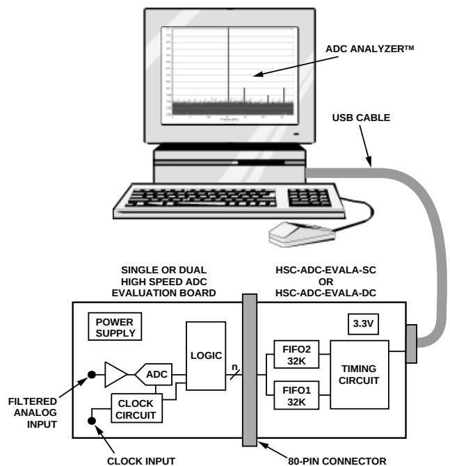
Figure 1. Functional Block Diagram (Simplified)
