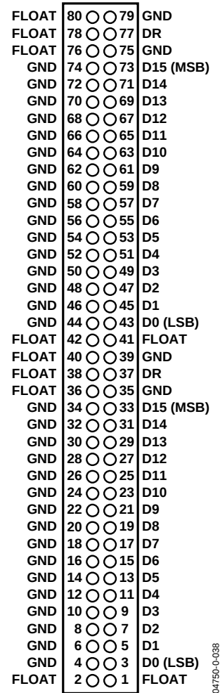
Figure 27. Dual-Channel Connector Pin Diagram— Top View (HSC-ADC-EVAL-DC)
