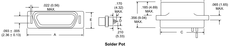
Solder Pot
