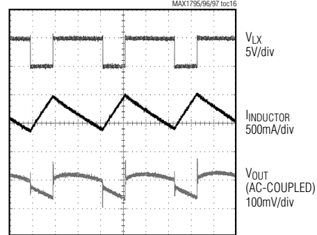
HEAVY-LOAD SWITCHING WAVEFORMS
