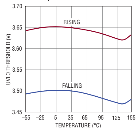
UVLO Threshold Voltages vs Temperature
