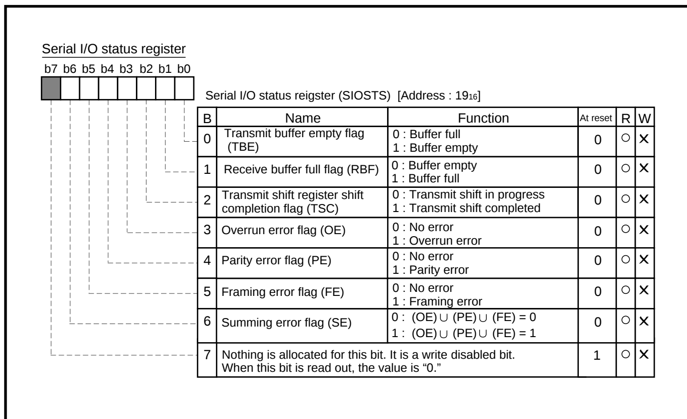
Fig. 2.3.3 Structure of Serial I/O status register
