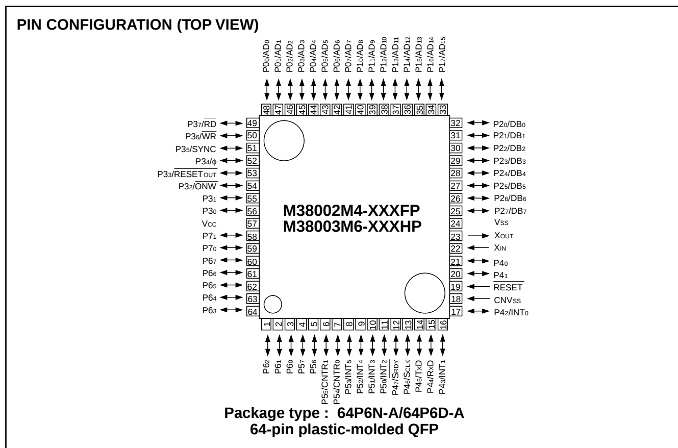
Fig. 1 Pin configuration of M38002M4-XXXXP/M38003M6-XXXXP
