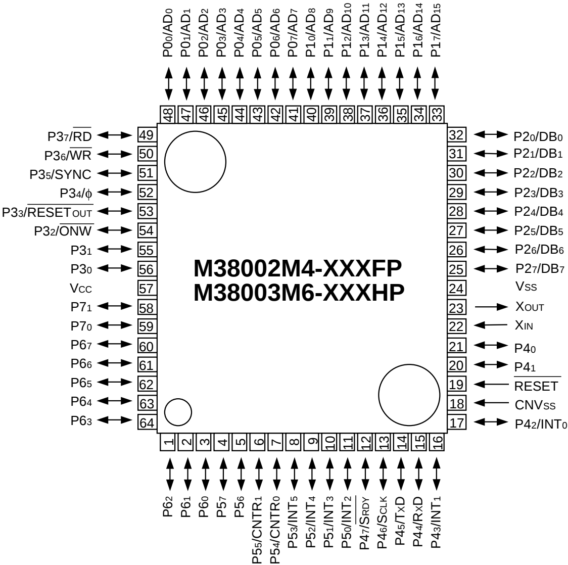
Package type : 64P6N-A/64P6D-A 64-pin plastic-molded QFP
