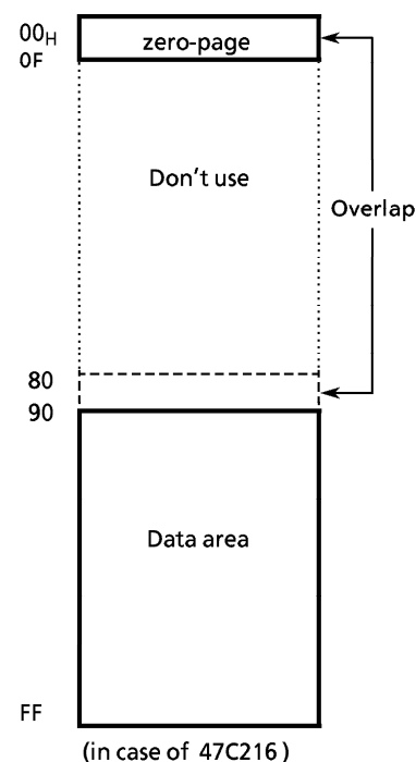
Figure 1-2. RAM addressing
