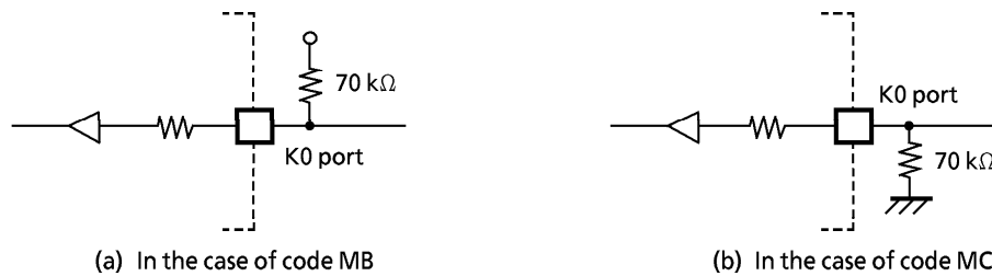
Figure 1-3. I/O Circuitry Code and External Circuitry
