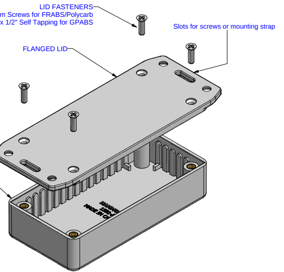
EXPLODED VIEW OF FLANGED ASSEMBLY
