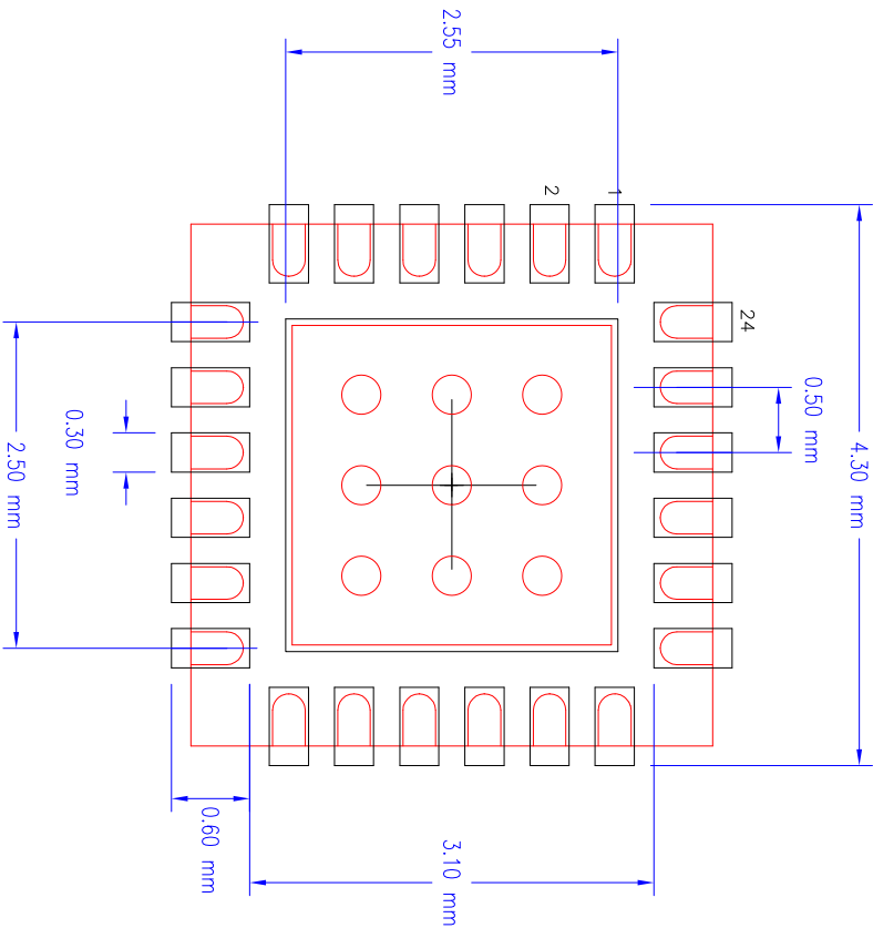
NLG24 RECOMMENDED FOOTPRINT 2.45 mm SQ EPAD
