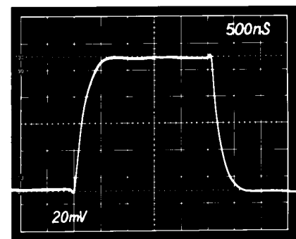
Figure 29c. Unity-Gain Inverter Small Signal Pulse Response
