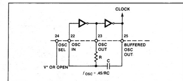
Figure 6. RC Oscillator
