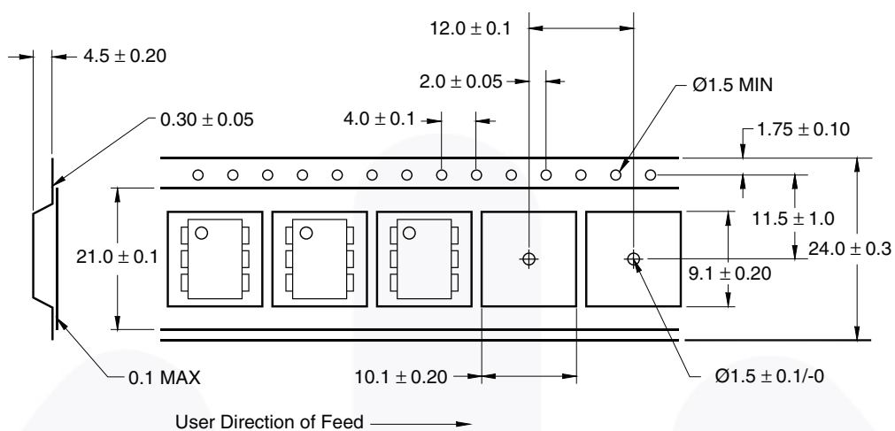
Figure 14. Tape Dimensions
