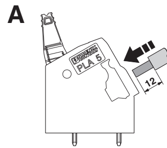
Functional drawing
