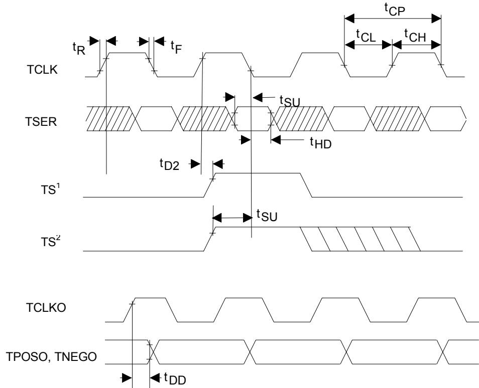
Figure 19-11. Transmit Timing, T1/E1
