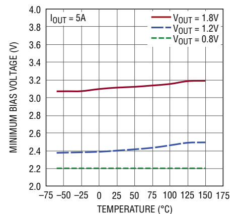
Minimum BIAS Voltage vs Temperature
