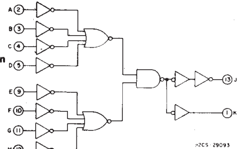
Fig. 1 – Logic diagram.
