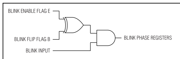
Figure 11. Blink Logic
