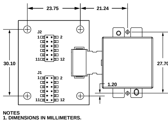
Figure 17. Physical Diagram for the ADIS16367/PCBZ
