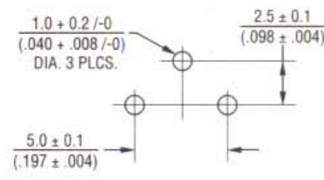
Suggested PCB Layout – Styles K, P, W
