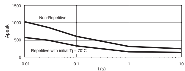
Figure 5b — DRD48D25
