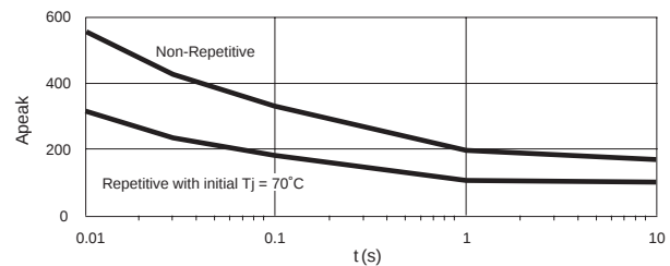
Figure 5a — DRD48X20
