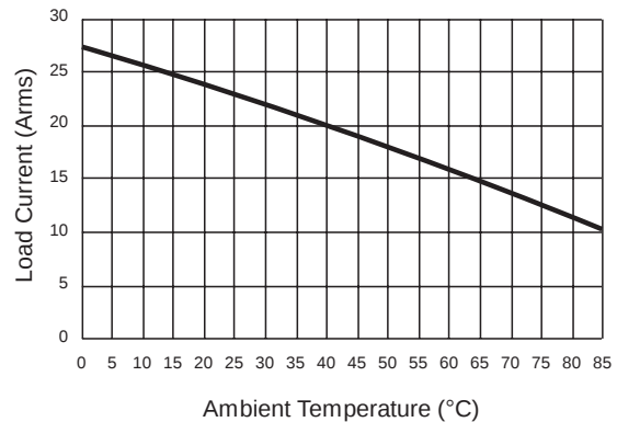
Figure 4a — DRD48X20
