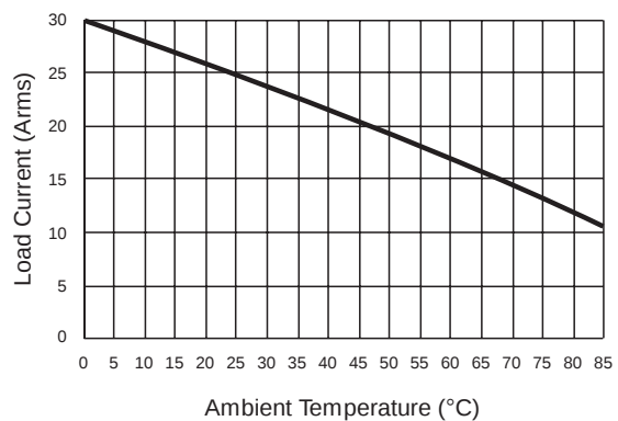
Figure 4b — DRD48D25
