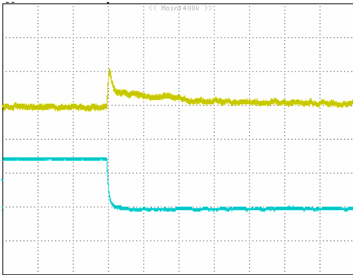
Figure 23: Typical transient response to step load change at 2.5\text{A}/\mu\text{S} from 100% to 0% of I_o , max at 5V_{in} , 1.8V_{out} (200uS/div) ( C_{out} = 47\mu\text{F} ceramic).top trace: V_{out} , 0.1V/div;bottom trace: I_{out} : 2A/div.
