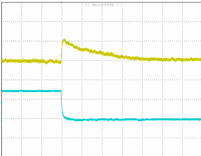
Figure 25: Typical transient response to step load change at 2.5\text{A}/\mu\text{S} from 100% to 0% of I_o , max at 5V_{in} , 3.3V_{out} (200uS/div) ( C_{out} = 47\mu\text{F} ceramic).top trace: V_{out} , 0.1V/div;bottom trace: I_{out} : 2A/div.
