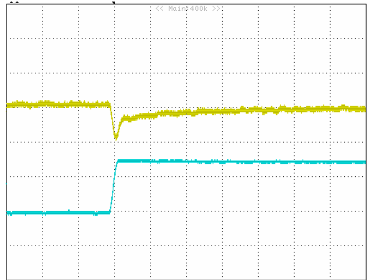
Figure 24: Typical transient response to step load change at 2.5\text{A}/\mu\text{S} from 0% to 100% of I_o , max at 5V_{in} , 1.8V_{out} (200uS/div) ( C_{out} = 47\mu\text{F} ceramic).top trace: V_{out} , 0.1V/div;bottom trace: I_{out} : 2A/div.
