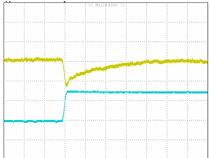
Figure 26: Typical transient response to step load change at 2.5\text{A}/\mu\text{S} from 0% to 100% of I_o , max at 5V_{in} , 3.3V_{out} (200uS/div) ( C_{out} = 47\mu\text{F} ceramic).top trace: V_{out} , 0.1V/div;bottom trace: I_{out} : 2A/div.
