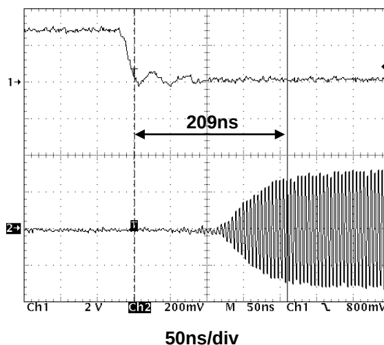
Switching Speed
