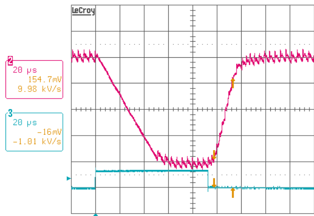
FIGURE 57. 1-PHASE GPU MODE VID TRANSITION, DPRSLPVR = 1, I_0 = 2A , VID = 1.2375V/1.0375V, Ch2: V_O , Ch3: VID4
