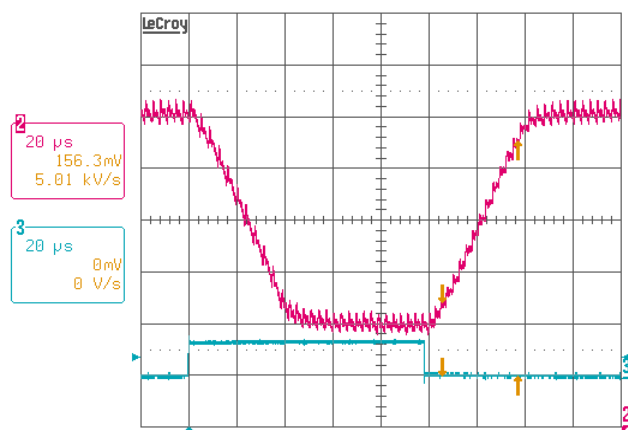
FIGURE 56. 1-PHASE GPU MODE VID TRANSITION, DPRSLPVR = 0, I_0 = 2A , VID = 1.2375V/1.0375V, Ch2: V_O , Ch3: VID4
