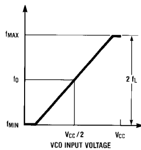
VCO WITHOUT OFFSET R_2 = \infty
