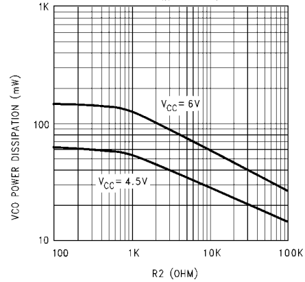
VHC4046 Typical VCO Power Dissipation @ f_{MIN} vs R_2
