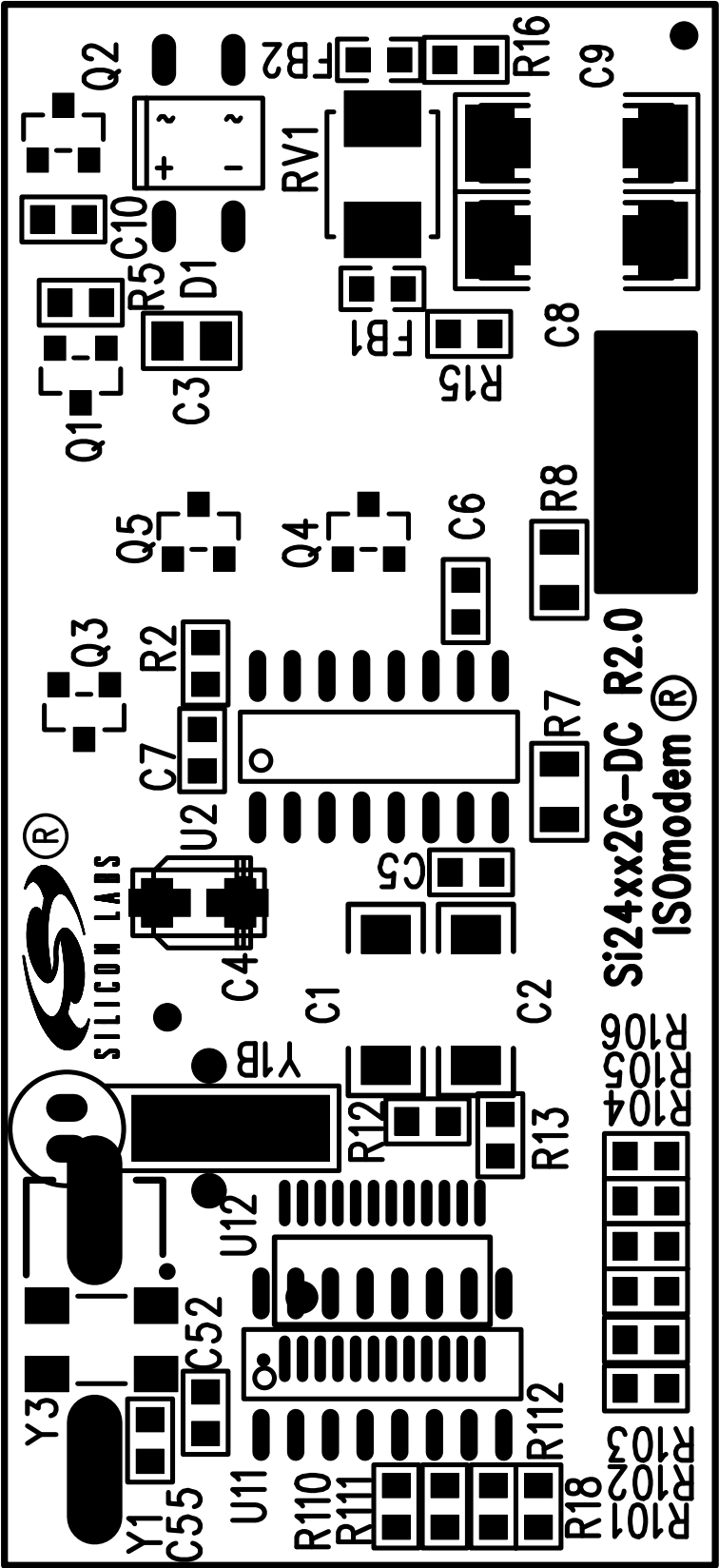
Figure 39. Daughter Card Primary Side, Component and Silkscreen
