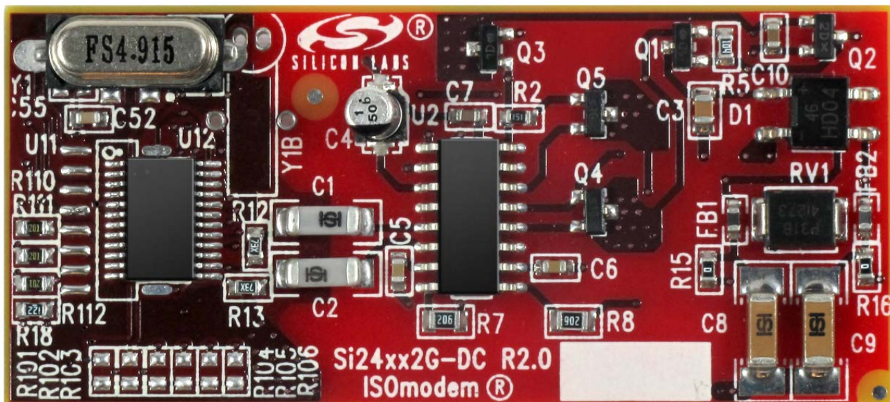
Figure 3. Daughter Card
