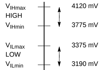
Figure 18. MC100EP116 Single-Ended Input Example
