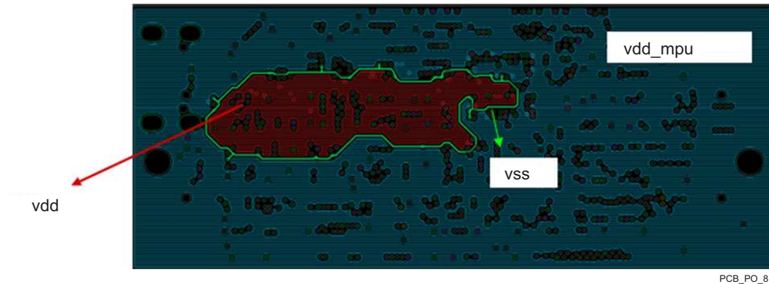
Figure 8-8. Coplanar Shielding of Power Net Using Ground Guard-band
