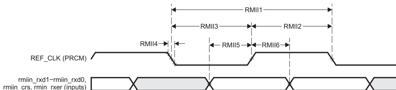
Figure 7-50. GMAC Receive Interface Timing RMII Receive operation
