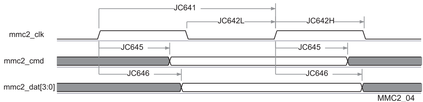
Figure 7-71. MMC/SD/SDIO in - High Speed JC64 - Transmitter Mode
