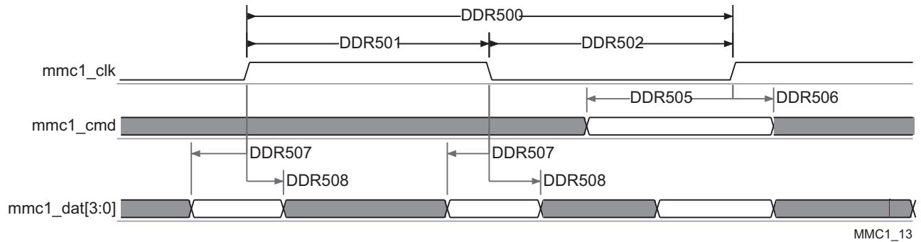
Figure 7-66. SDMMC - High Speed SD - DDR - Data/Command Receive
