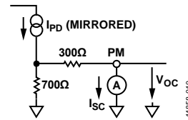
Figure 10. Typical PM Circuit and Test Setup
