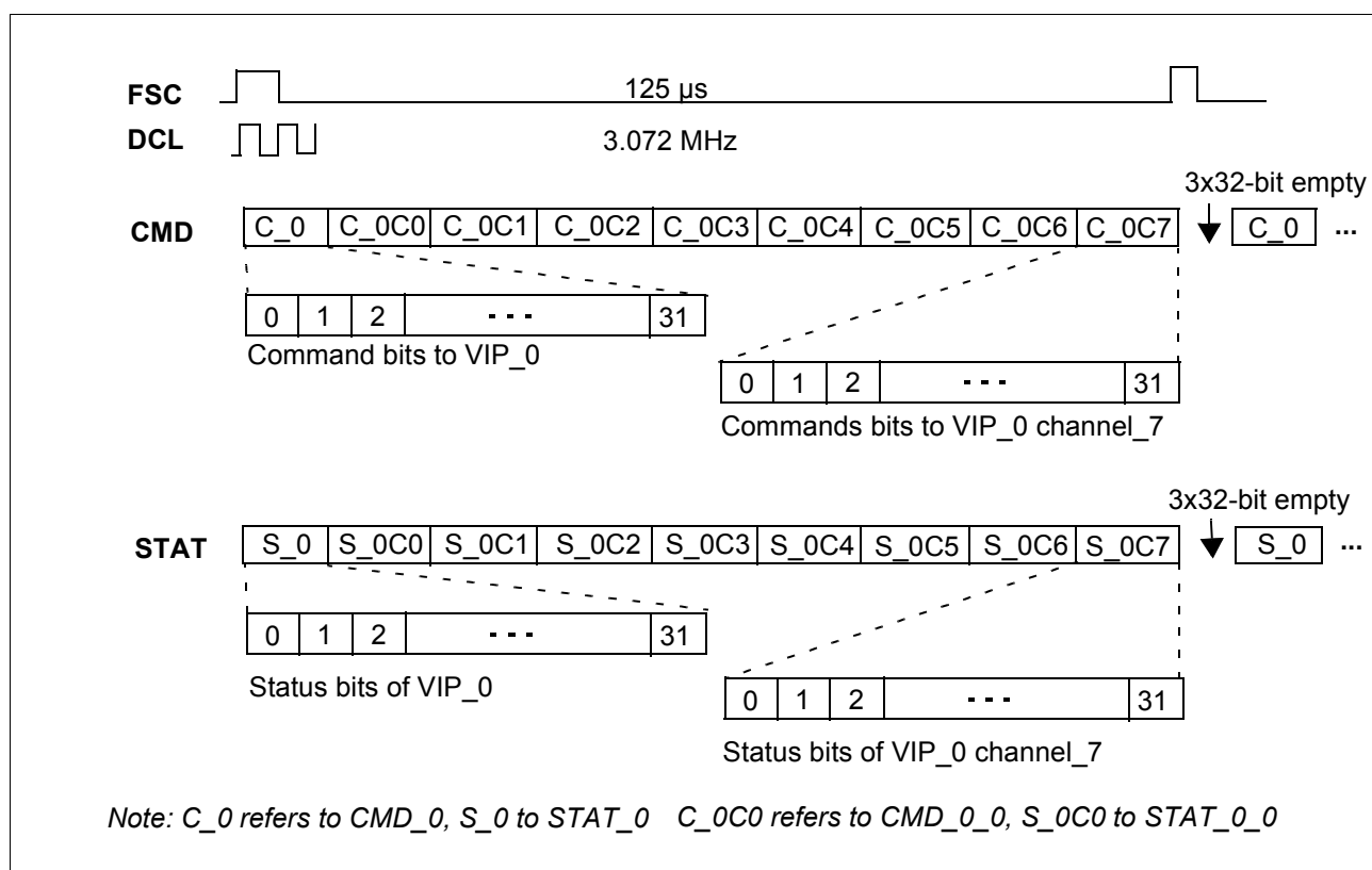
Figure 14 IOM-2000 CMD/STAT Handling (1 VIP with 8 Channels)
